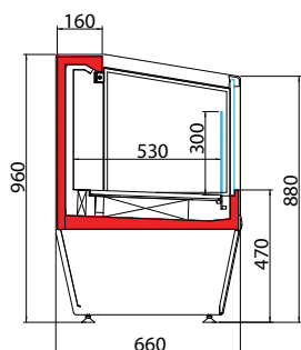
DOORSNEDE PLANET2
